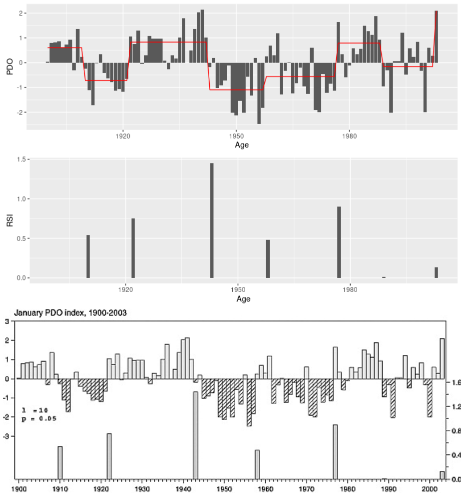
Figure 1: The RSI plot generated by rshift , and the plot of the same data from Rodionov [2004].
